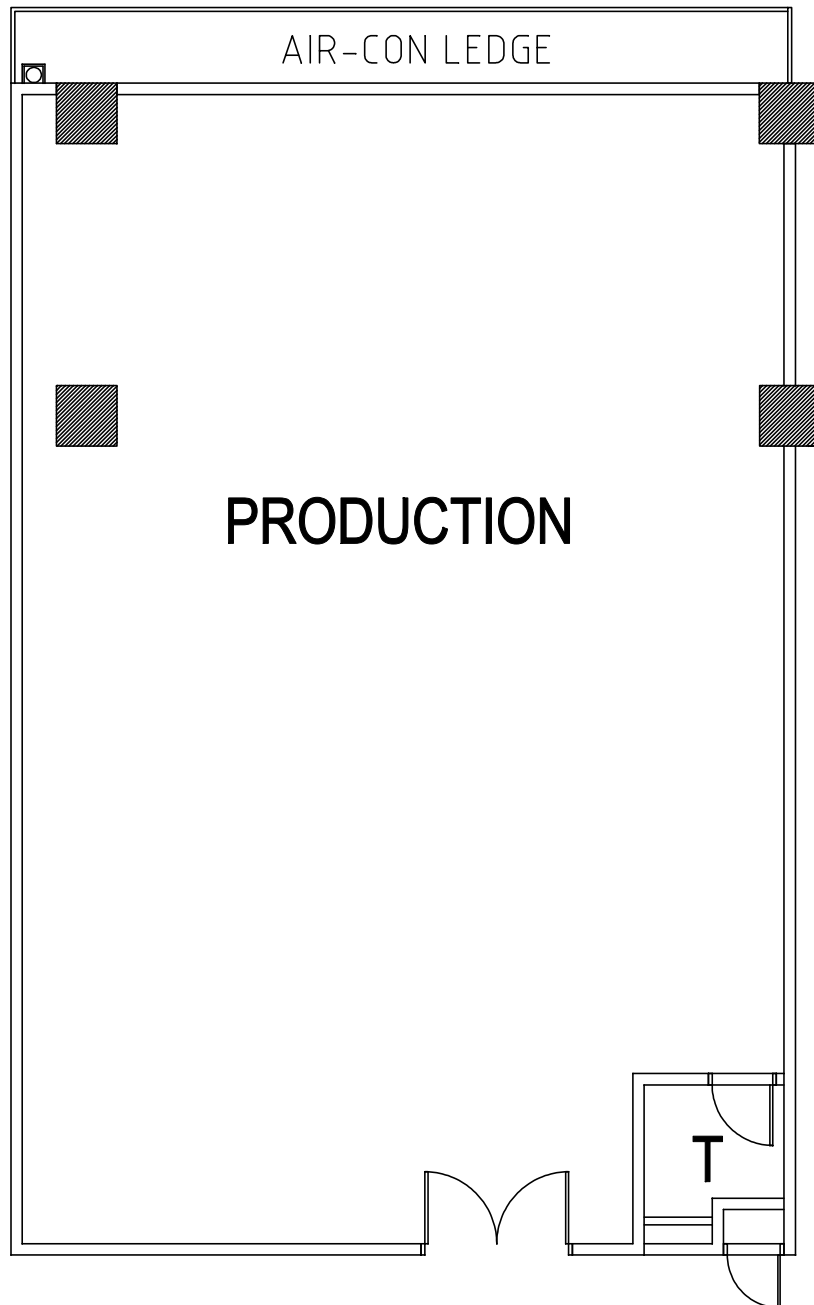
TYPE A15 – TYPICAL 6TH TO 9TH STOREY PLAN SCALE 1:100
