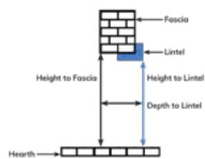
Fascia and Lintel Dimensions
