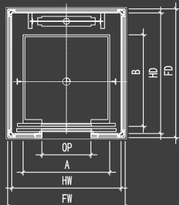
Hoistway Plan
