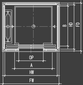
Hoistway Plan
