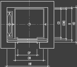
Hoistway Plan
