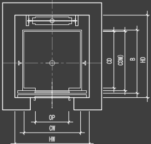
Hoistway Plan
