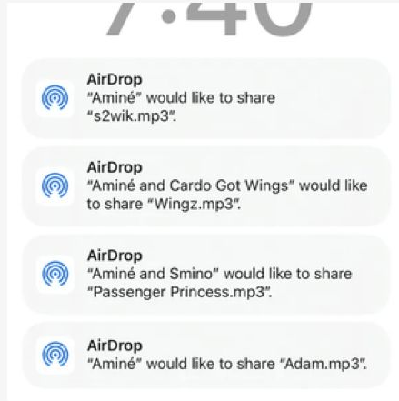
s2wik - Amine
