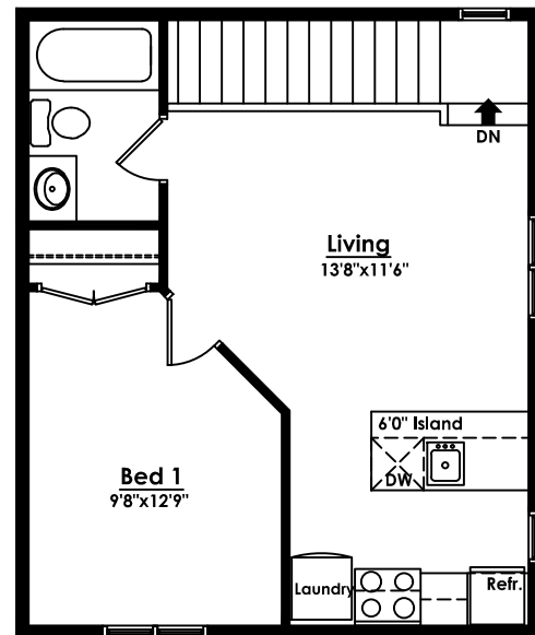
Second Floor Plan 480 sf
