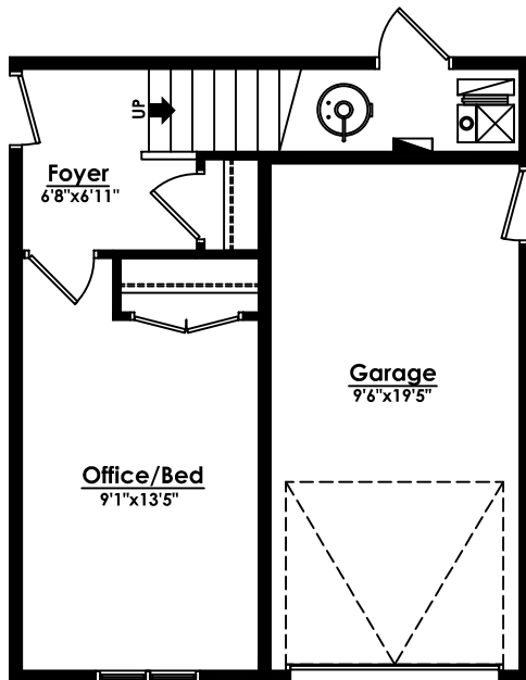
Main Floor Plan 480 sf
