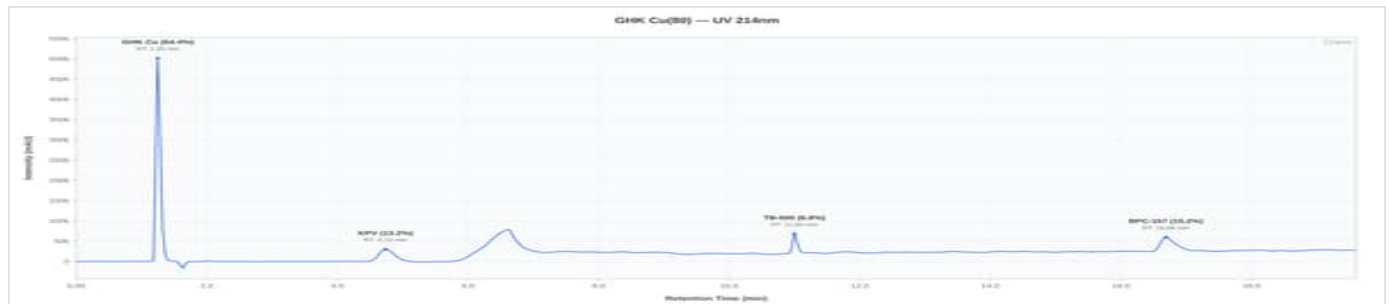
KLOW 80 - AEON-KLO80-C1726: UV Chromatogram
