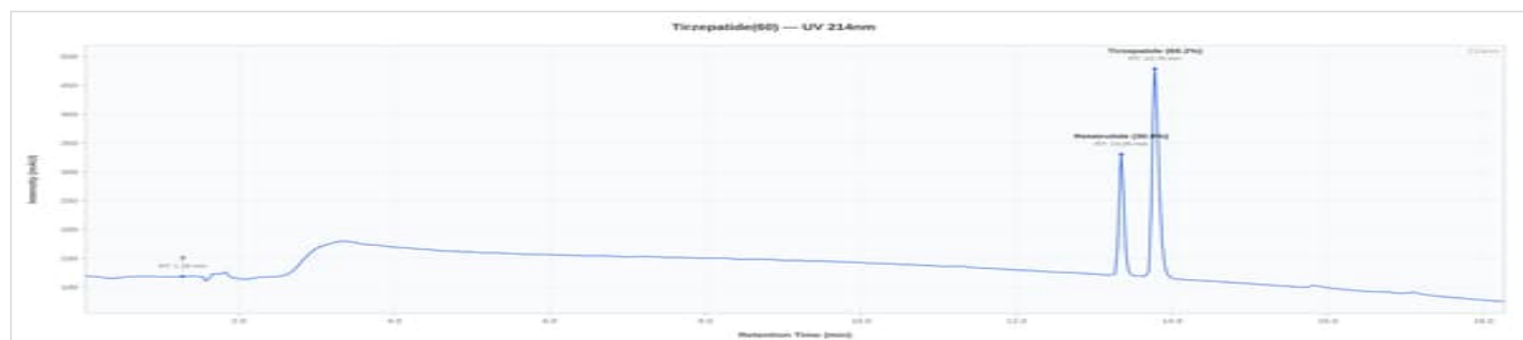
R-T FUSION 60 - AEON-RET60-C1726: UV Chromatogram
