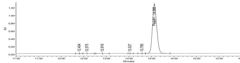
HPLC-UV Chromatogram
