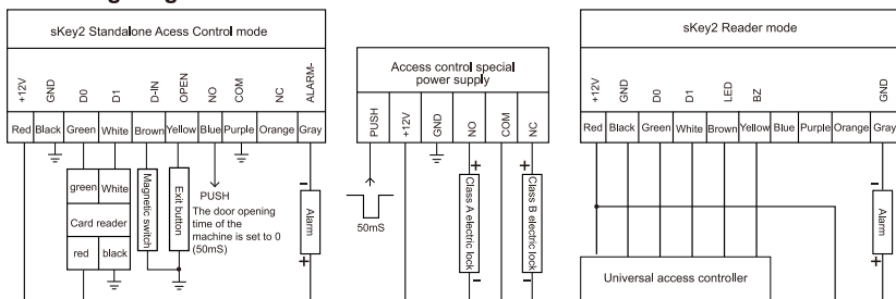
Wiring Diagram
