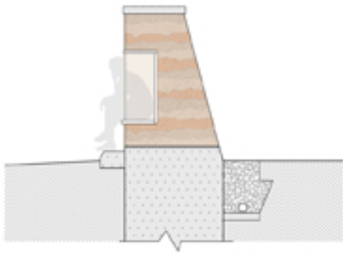
4. Rammed earth walls with seating
