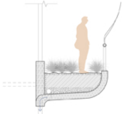
3. Harvest tower planter detail
