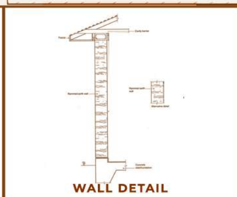
WALL DETAIL
